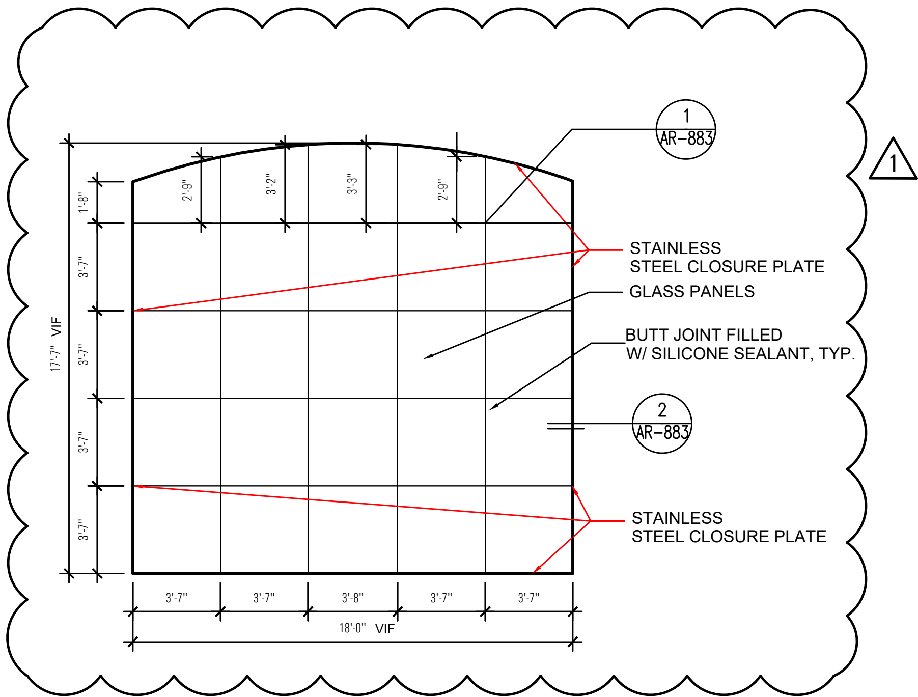
2 ELEVATION NORTH EOP - ARTWORK LOCATION #2 - PANEL GRID ARTIST: TOMIE ARAI 1/4" = 1'-0"
