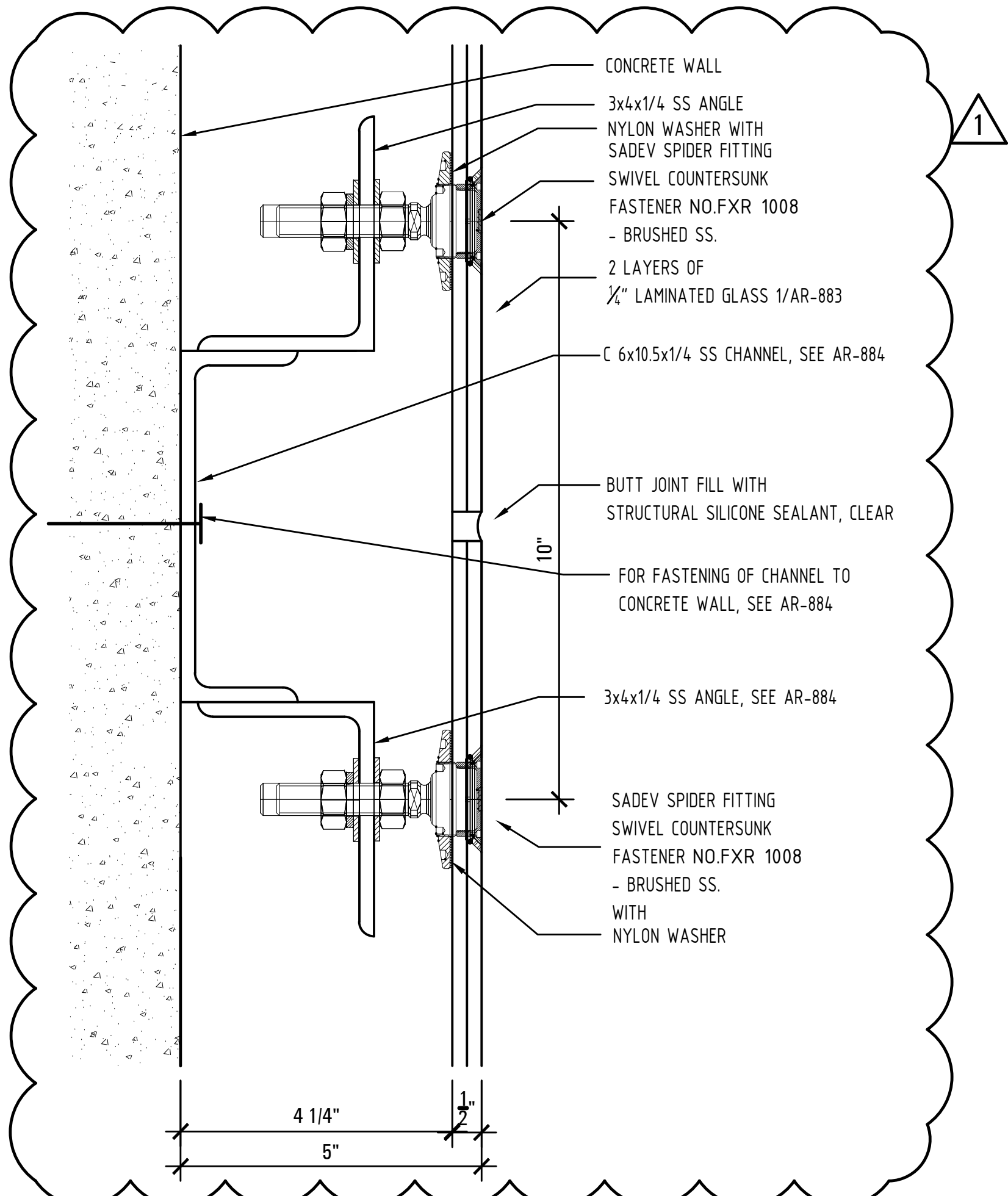
3 DETAIL OF ART GLASS ASSEMBLY - MOUNTING FASTENERS - INTERIOR CONCRETE WALL CONDITION 6" = 1'-0" SCALE
