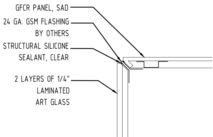
4 ART GLASS AND GFR PANEL CONNECTION AT CORNER 3"=1'-0" NOTE: MOUNTING CONDITIONS VARY - SEPARATE DETAILS TO BE INCLUDED IN DRAWINGS BASED UPON MANUFACTURER'S RECOMMENDATIONS.
