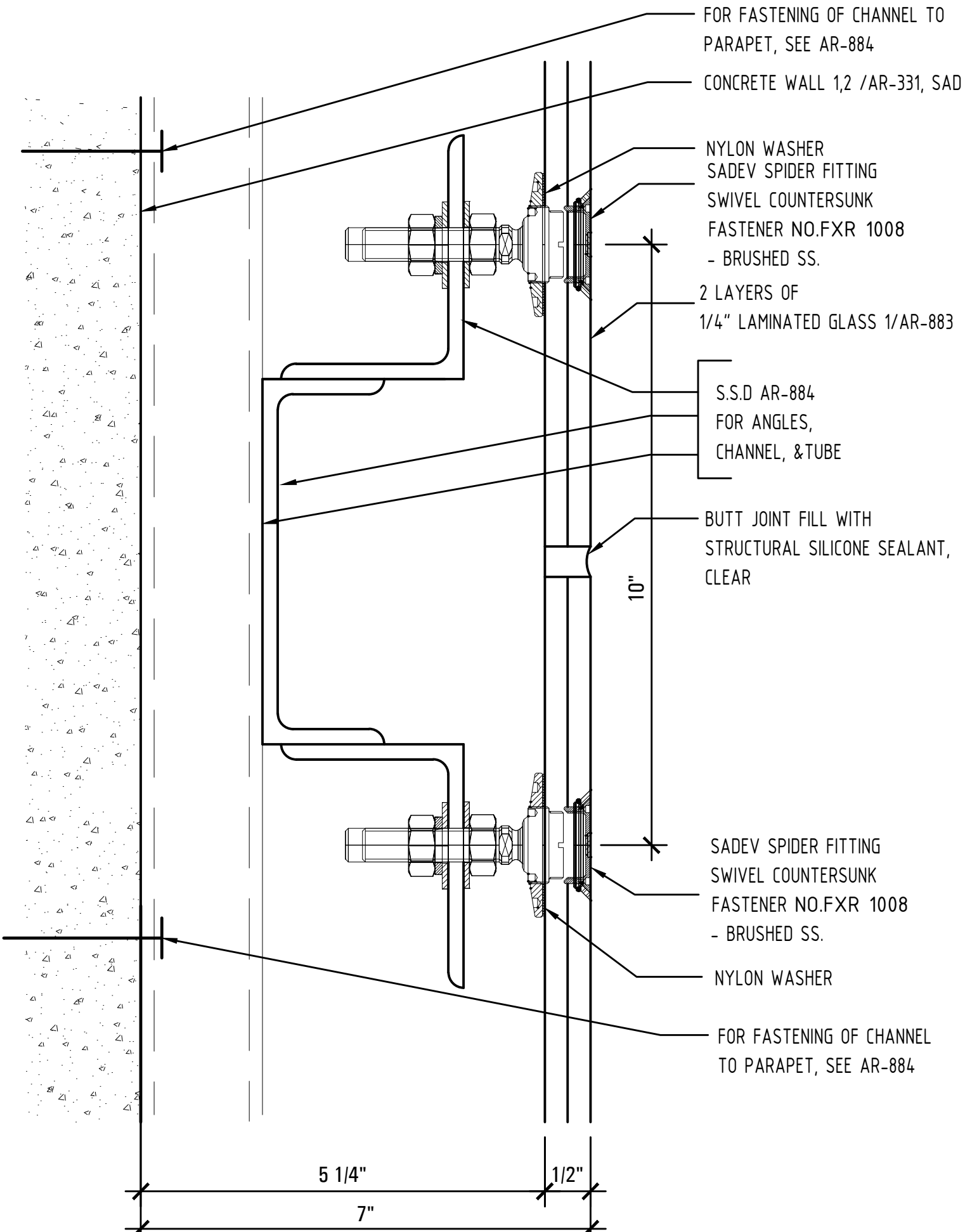
6 DETAIL OF ART GLASS ASSEMBLY - MOUNTING FASTENERS - PARAPET CONDITION 6"=1'-0" NOTE: MOUNTING CONDITIONS VARY - SEPARATE DETAILS TO BE INCLUDED IN DRAWINGS BASED UPON MANUFACTURER'S RECOMMENDATIONS.
