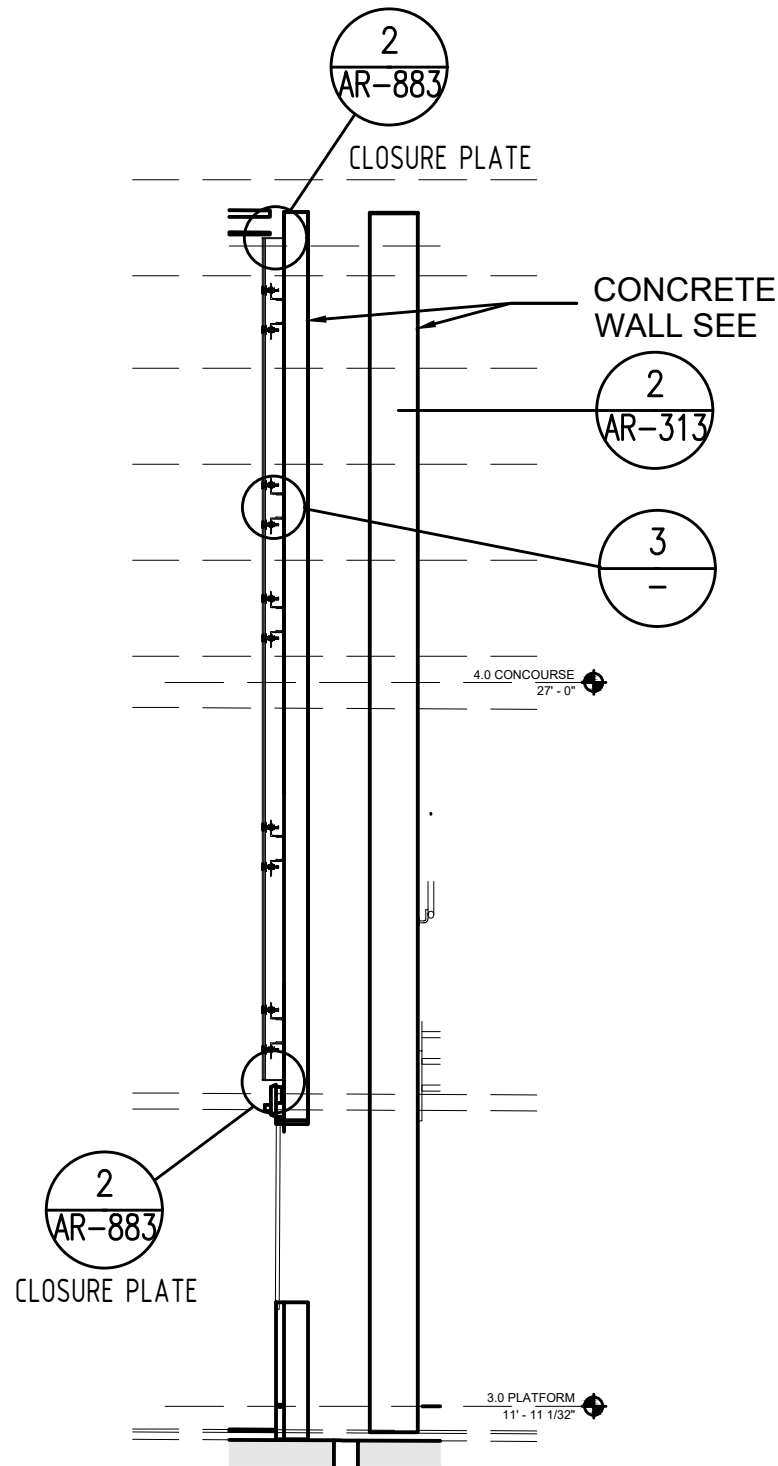
4 SECTION SOUTH WALL EOP - ARTWORK LOCATION #3B ARTIST: TOMIE ARAI
