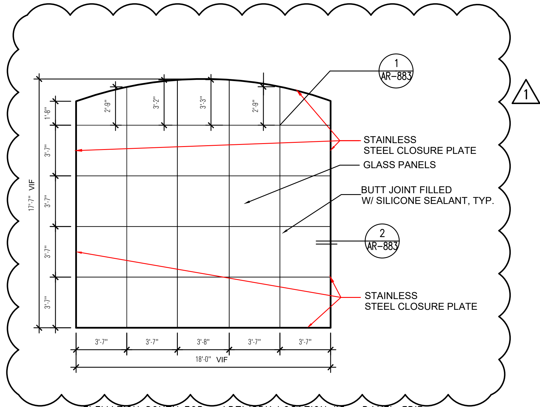
2 ELEVATION SOUTH EOP - ARTWORK LOCATION #3 - PANEL GRID ARTIST: TOMIE ARAI
