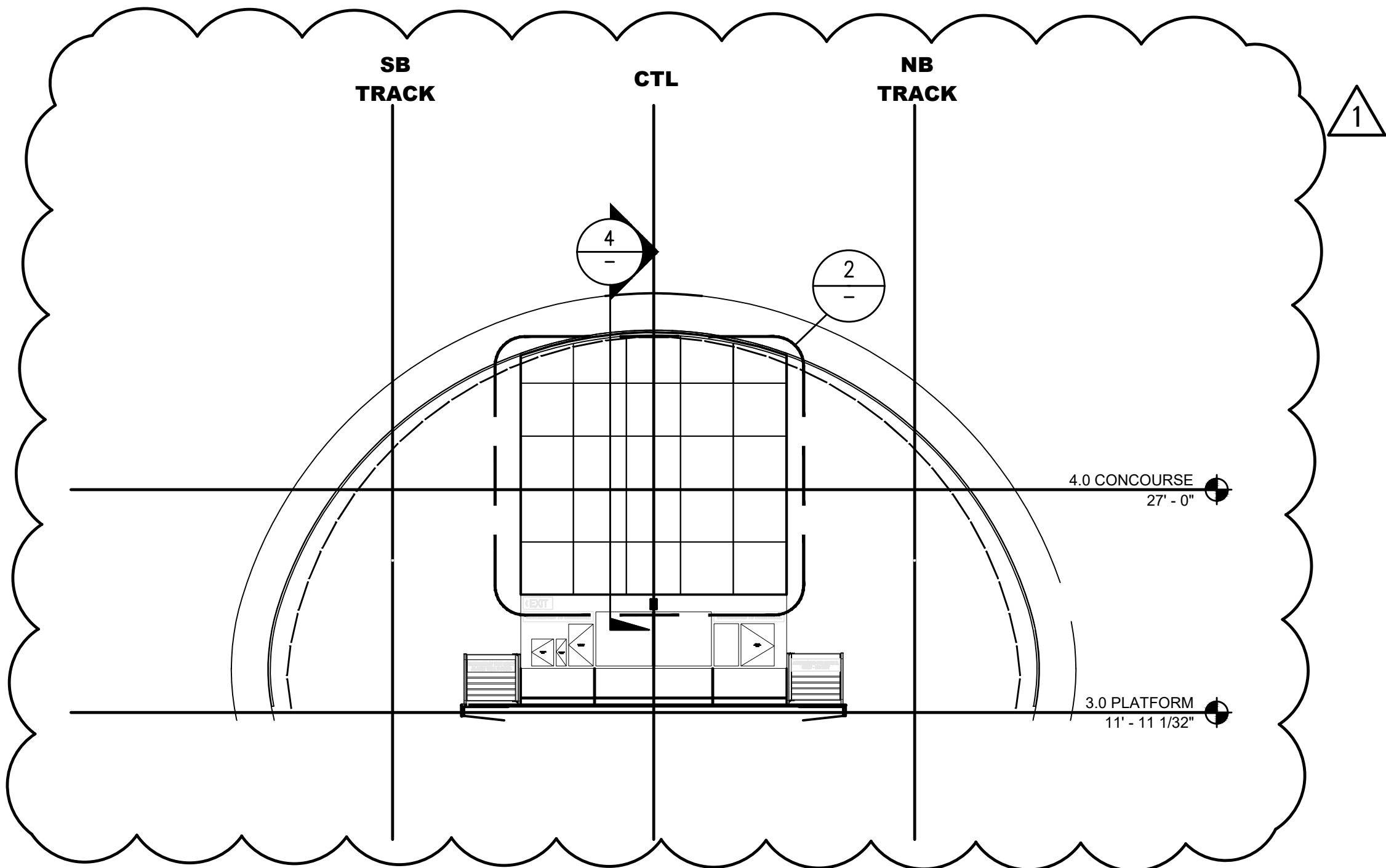
1 ELEVATION NORTH EOP- ARTWORK LOCATION #2 ARTIST: TOMIE ARAI 1/8" = 1'-0"
