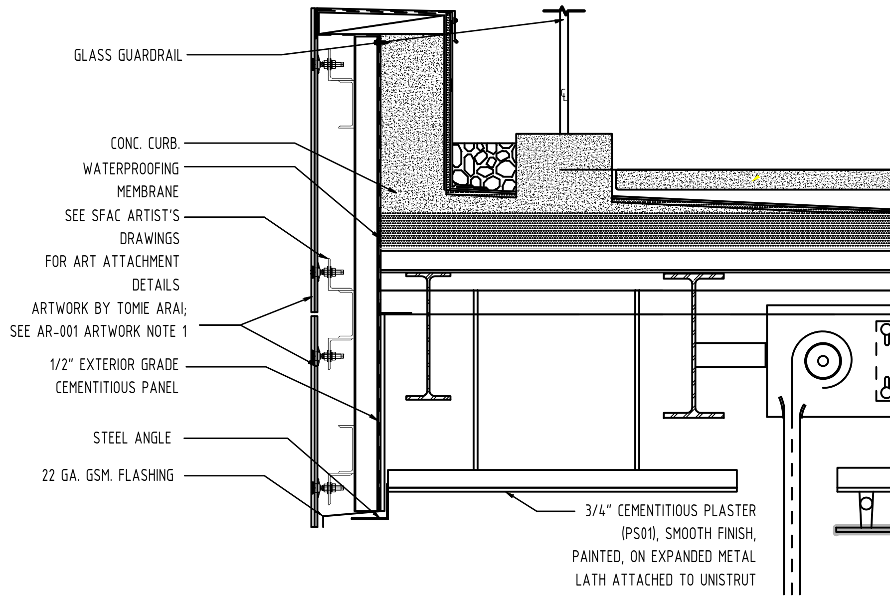
2 STOCKTON STREET ELEVATION - ARTWORK LOCATION #1B - CURB MOUNTING DETAIL ARTIST: TOMIE ARAI 1" = 1'-0"
