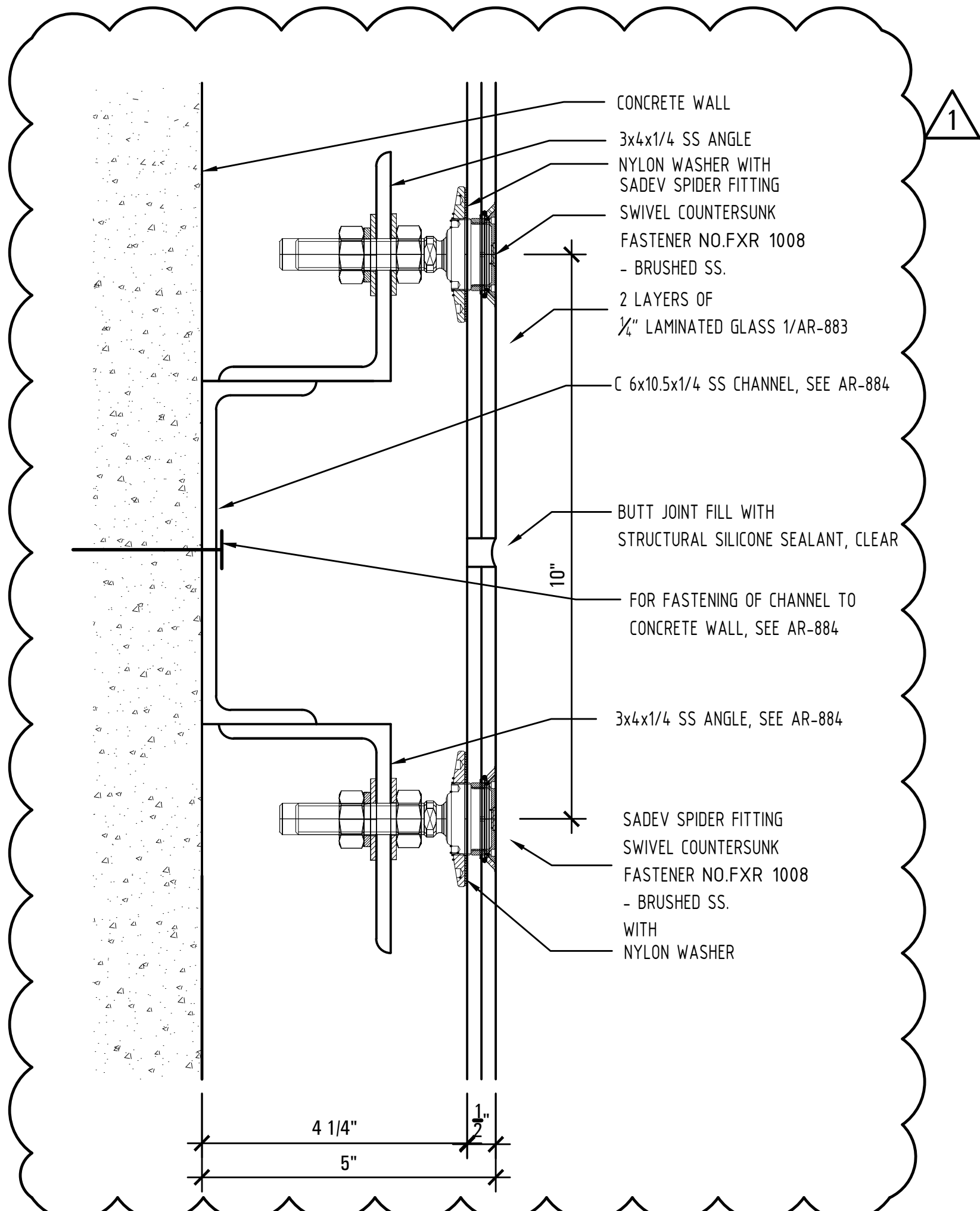
3 DETAIL OF ART GLASS ASSEMBLY - MOUNTING FASTENERS - INTERIOR CONCRETE WALL CONDITION 6" = 1'-0" SCALE
