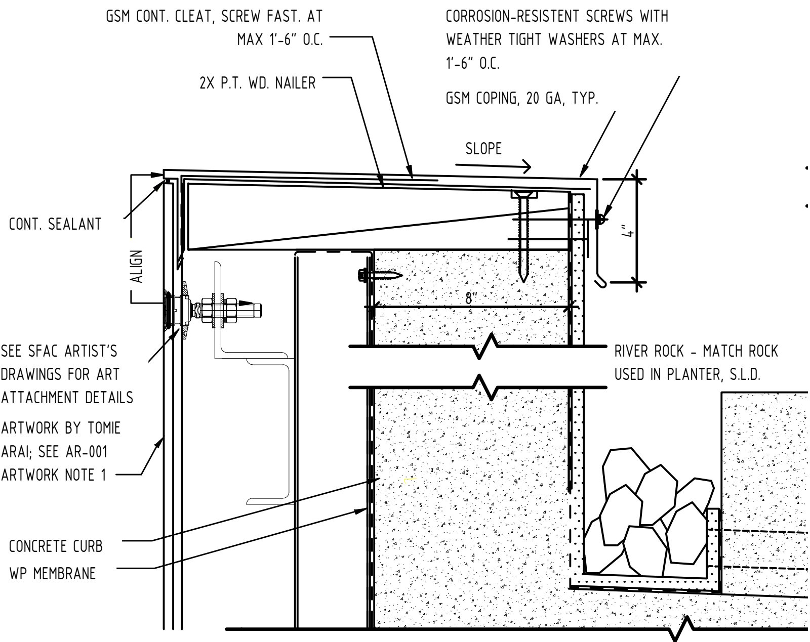
3 GSM FLASHING - PARAPET CONDITION 3"=1'-0" NOTE: MOUNTING CONDITIONS VARY - SEPARATE DETAILS TO BE INCLUDED IN DRAWINGS BASED UPON MANUFACTURER'S RECOMMENDATIONS.
