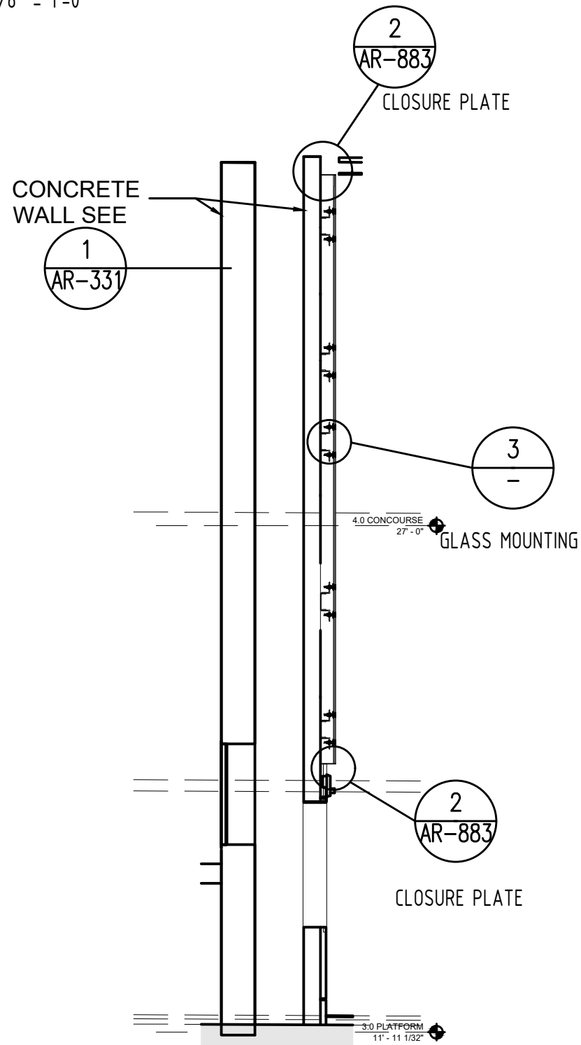
4 SECTION NORTH WALL EOP - ARTWORK LOCATION #2 ARTIST: TOMIE ARAI 1/4" = 1'-0"
