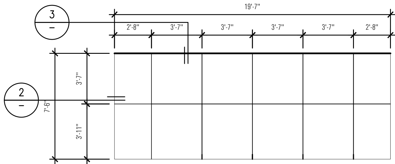
1 SOUTH PLAZA STREET ELEVATION - ARTWORK LOCATION #1C - PANEL GRID ARTIST: TOMIE ARAI 1/4" = 1'-0"
